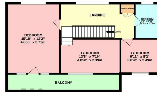
1ST FLOOR
